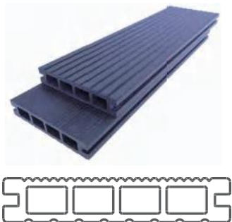
135H25-B 135*25 mm
